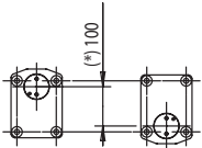
Alternative mounting position tilting kit
