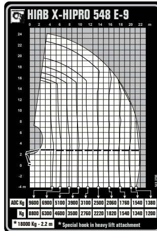
Lastdiagramm HIAB X-HIPRO 548 E-9
