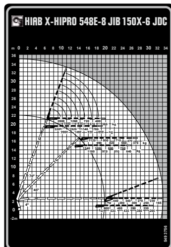
Lastdiagramm HIAB X-HIPRO 548 E-8 + JIB 150X-6 JDC
