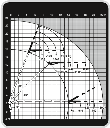
Diagramme de charge HIAB X-HIPRO 352 E-5 JIB 100X-3
