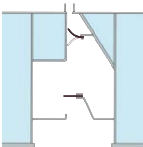
Double rubber lip seal
