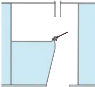
Open joint with drainage
