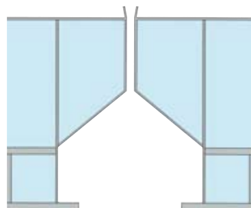
Open joint, no drainage
