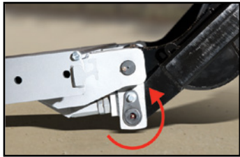
Simplified rocking pivot hinge reduces damage to concrete or asphalt that rollers may cause.
