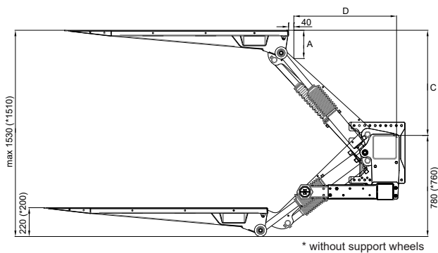
Installation dimensions (mm)
