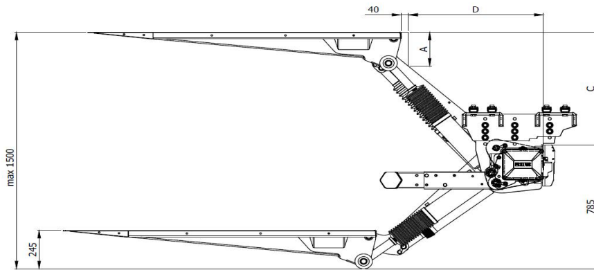
Installation dimensions (mm)
