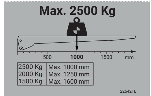
Loading diagram
