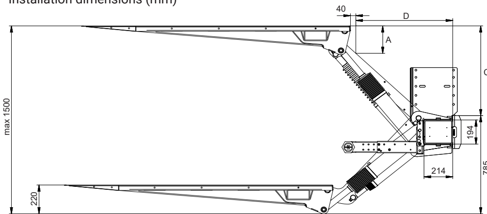
Installation dimensions (mm)
