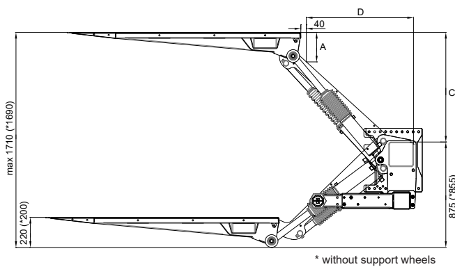
Installation dimensions (mm)
