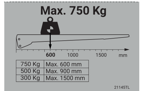
Loading diagram
