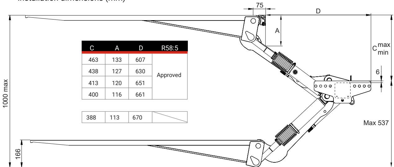
Installation dimensions (mm)
