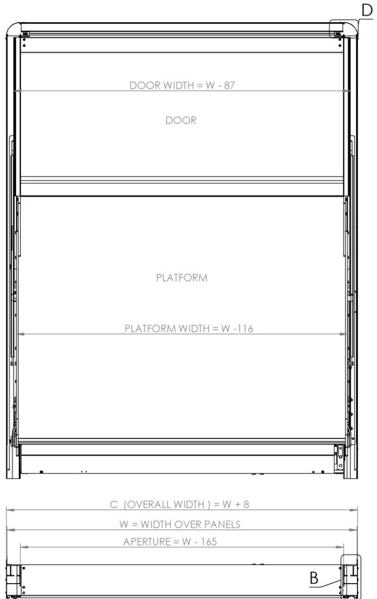
DETAIL C
