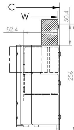
DETAIL B
