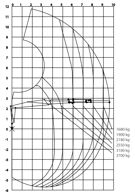
Lastdiagramm F140S 96i BOOSTER
