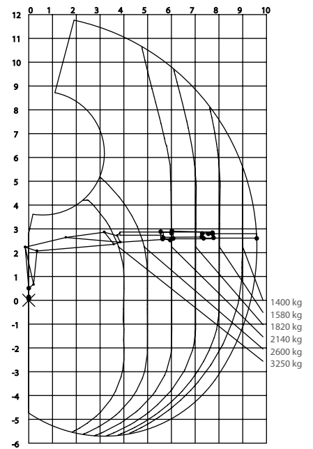
Lastdiagramm F140S 96i
