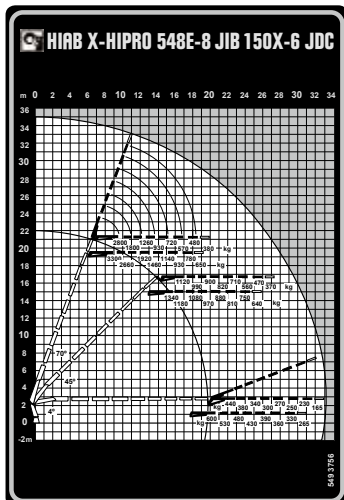
Lastediagram HIAB X-HIPRO 548 E-8 + JIB 150X-6 JDC
