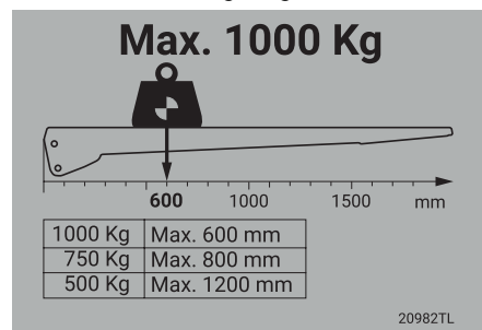
Loading diagram
